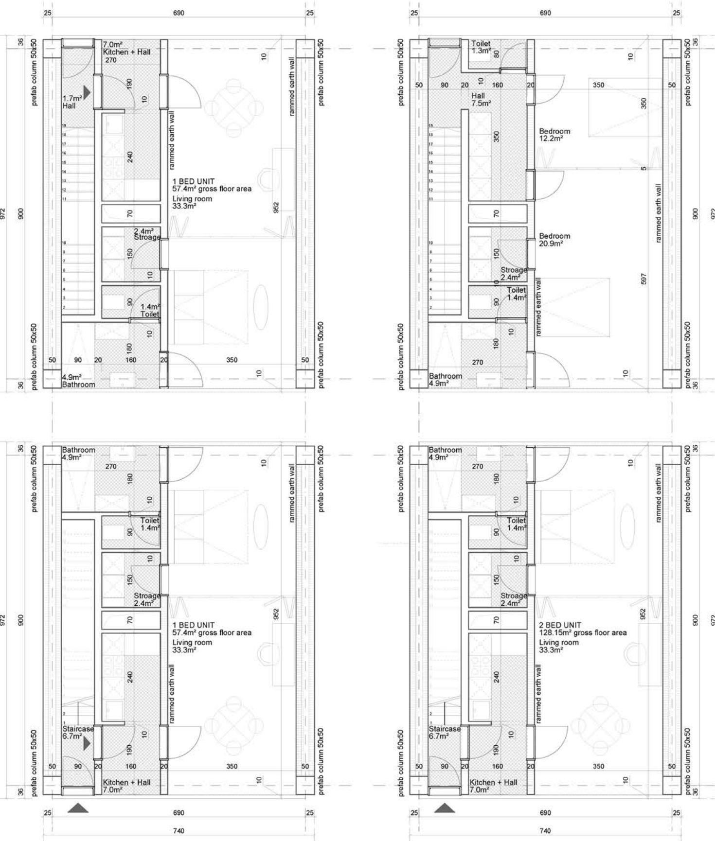
Detailed plan of living units
